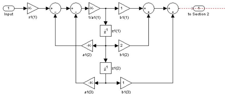
df2sos (Direct-form II, second-order sections)
